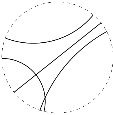
FIGURE 5.8. Geodesics of the Poincaré ball.
