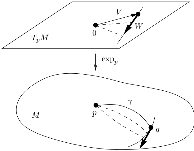
FIGURE 10.9. Computing (\exp_p)_*W .
