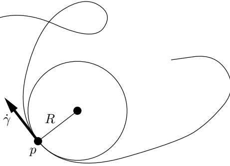
FIGURE 1.1. Osculating circle.
