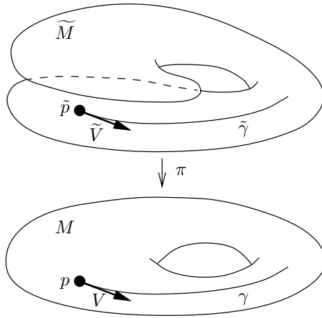
FIGURE 11.1. Lifting geodesics.
