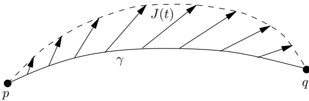
FIGURE 10.8. Conjugate points.
