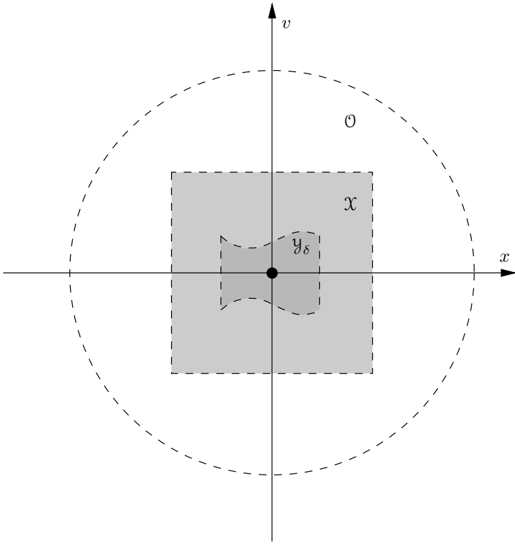
FIGURE 5.6. The sets Y_\delta \subset X \subset O .
