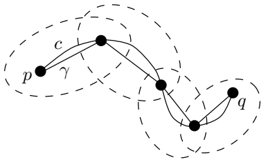
FIGURE 6.1. Any two points can be connected by an admissible curve.
