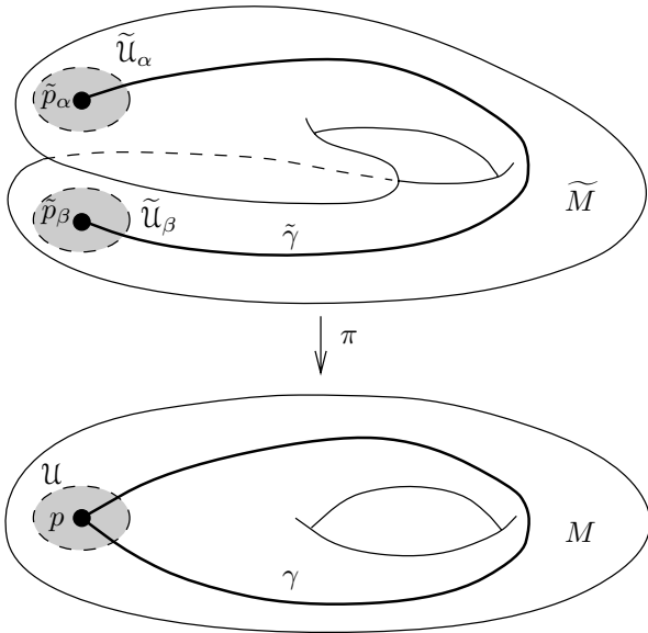
FIGURE 11.2. Proof that \tilde{U}_\alpha and \tilde{U}_\beta are disjoint.
