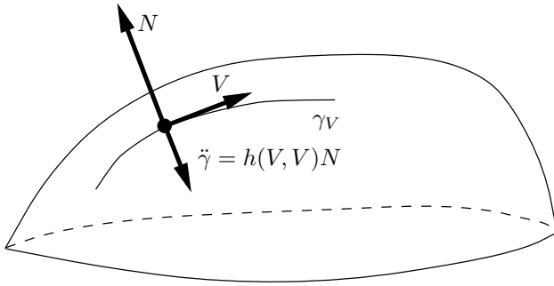
FIGURE 8.3. Geometric interpretation of h(V, V) .
