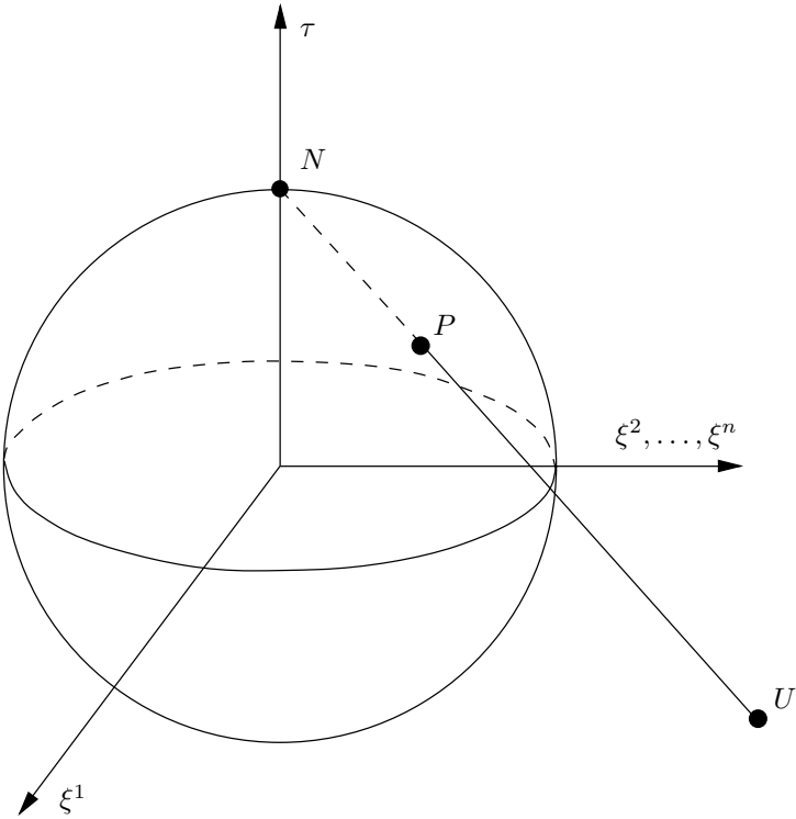
FIGURE 3.3. Stereographic projection.
