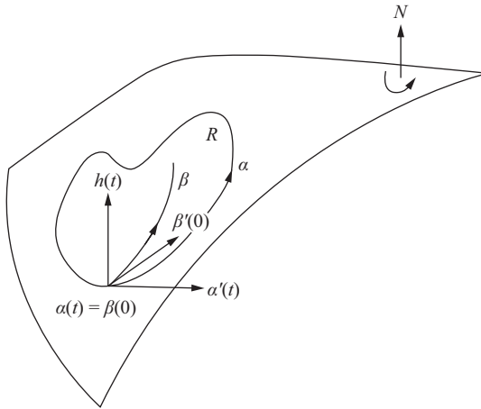
Figure 4-27. A positively oriented boundary curve.
