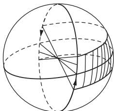
Figure 5.52. The projective plane contains a Möbius strip.
