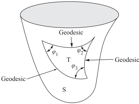
Figure 4-23. A geodesic triangle.
